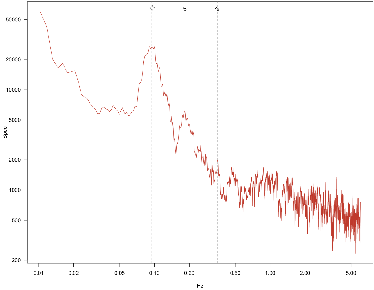
Figure 7: MTM power spectrum of Sunspot
